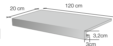
GRADINO LINEARE COSTA RETTA 20x120x3,2x3 - 8"x47"x1"x1.2"
